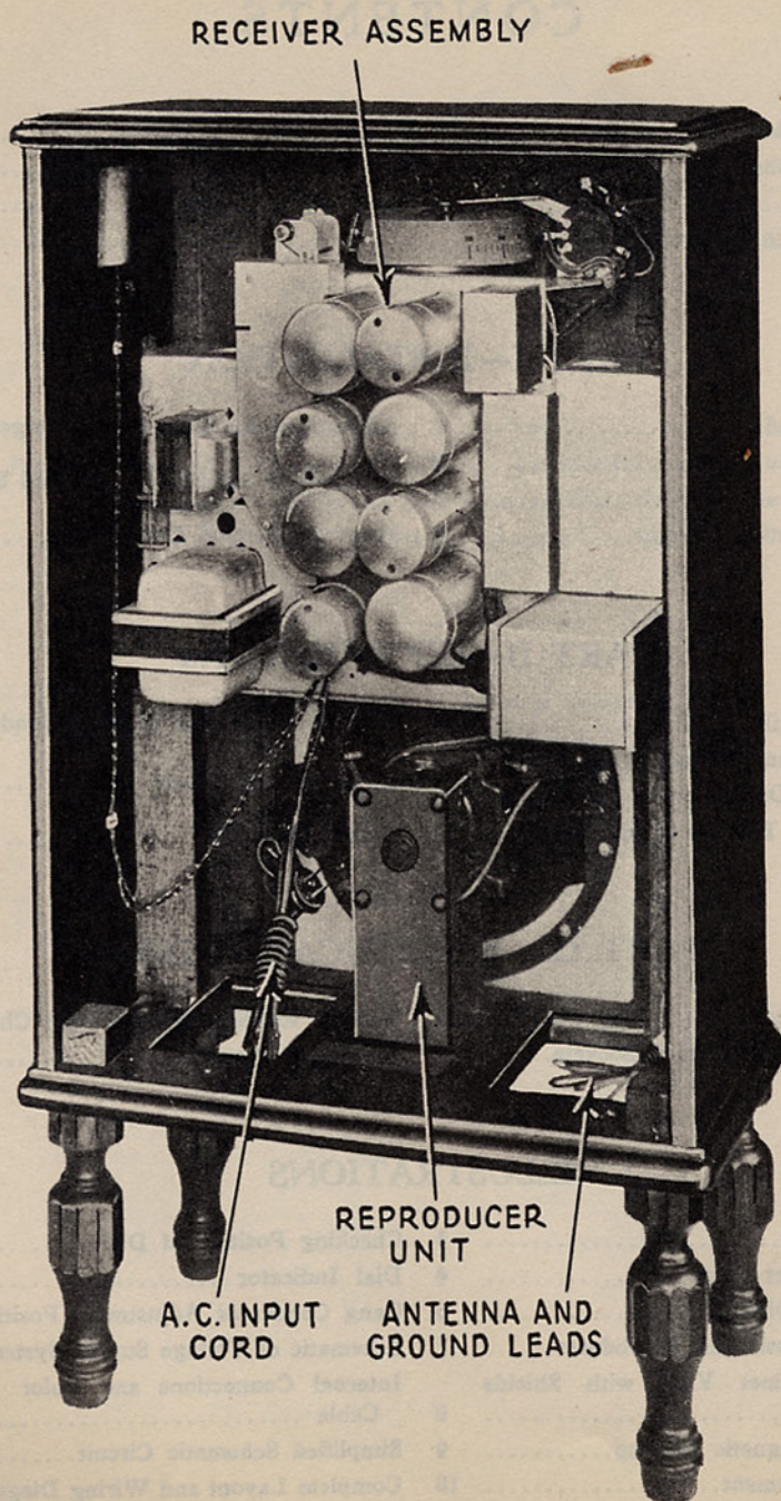
Figure 1—Rear interior cabinet view
