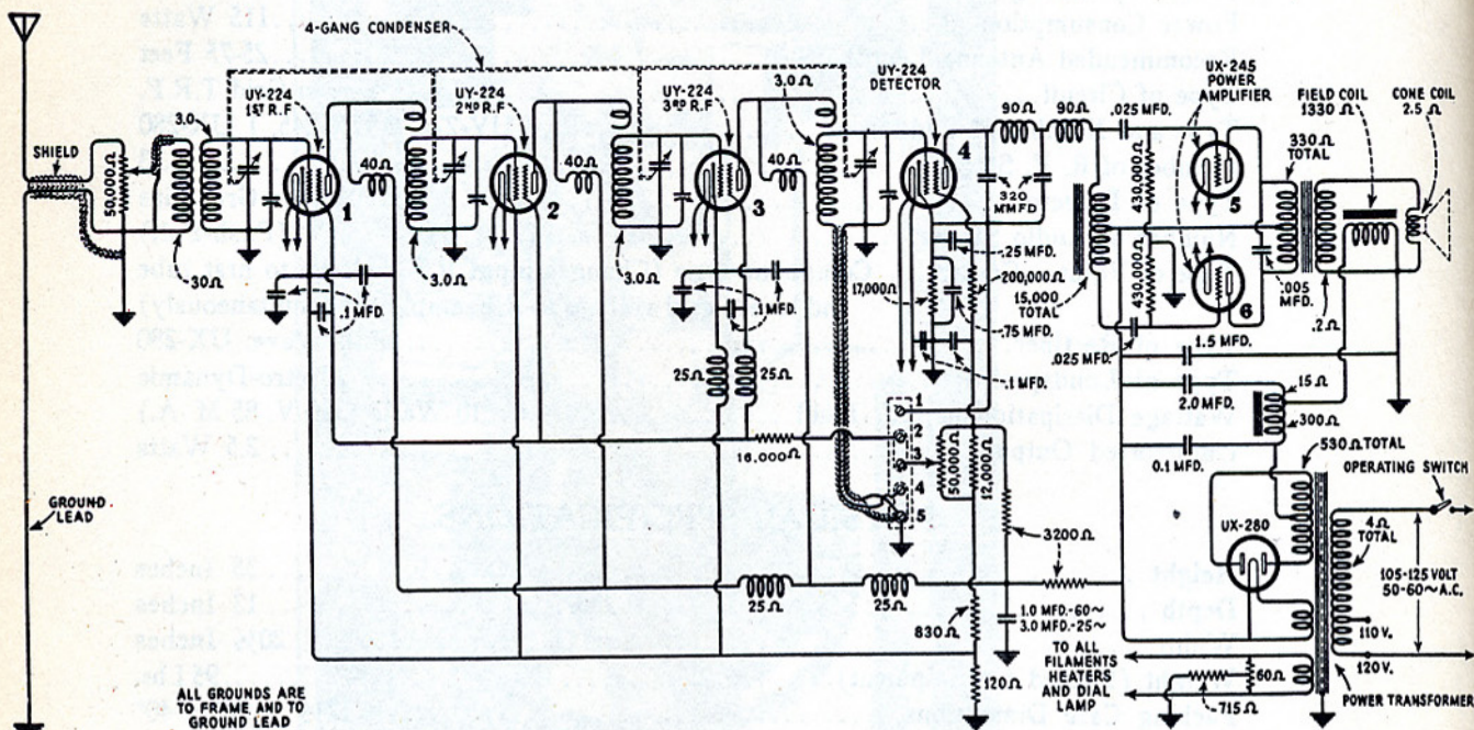
Figure 2—Schematic circuit diagram.
