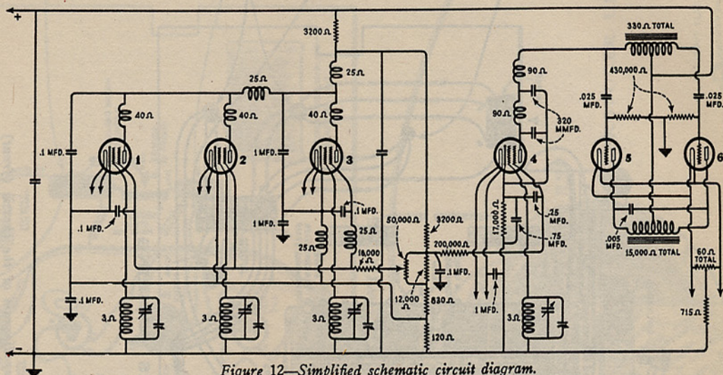
Figure 12—Simplified schematic circuit diagram.
